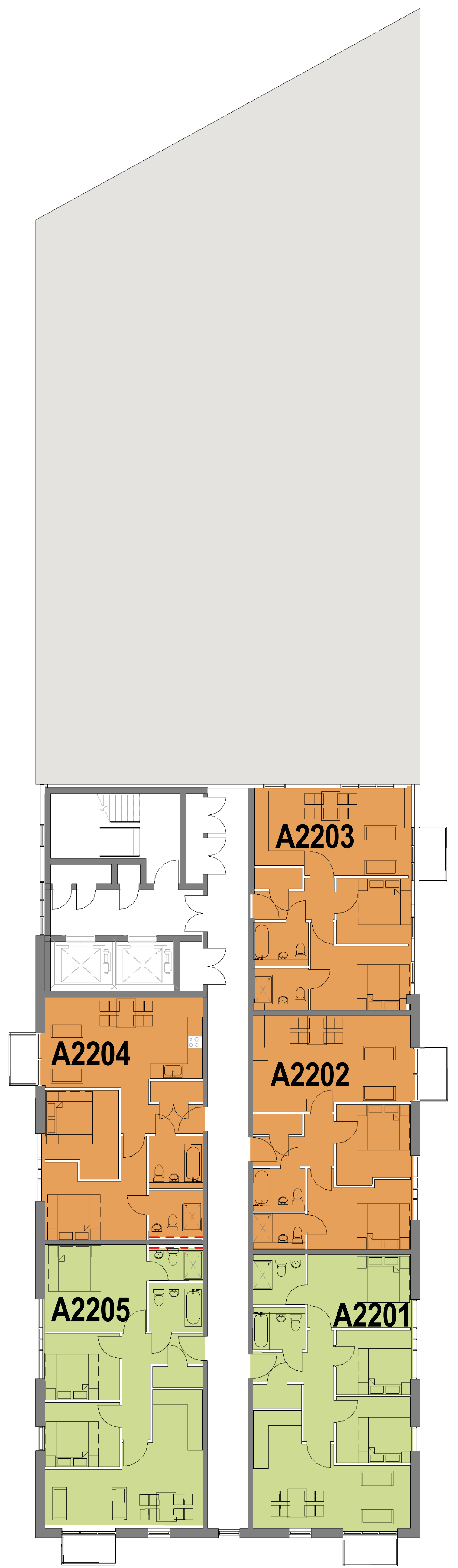
1 Block A - Twenty Second Floor 1 : 100
